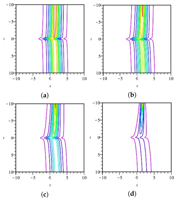
Figure 6. (a–d) The contour plots of the imaginary part of (43), in the z-axis orientation, for \mathfrak{B} = 0.10, 0.15, 0.20, 0.25 .
